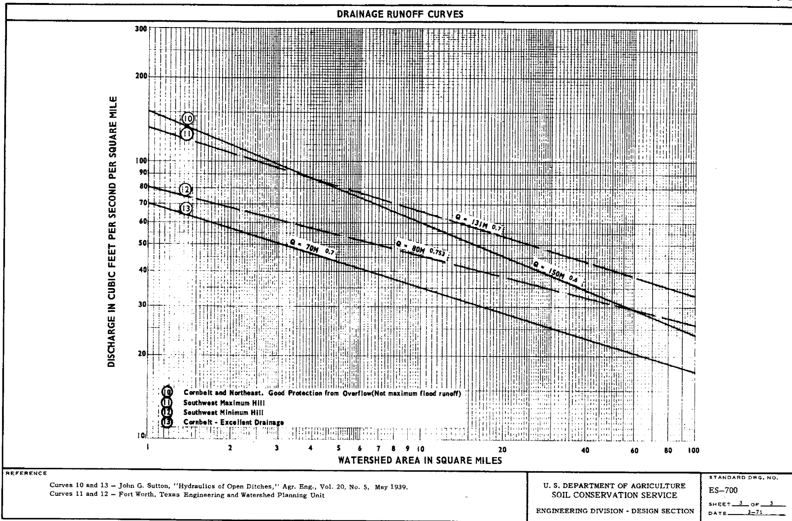
Figure 5-3, Drainage runoff curves
