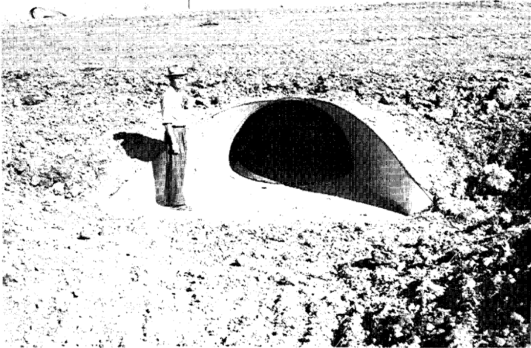
Prefabricated entrance section on pipe drop
